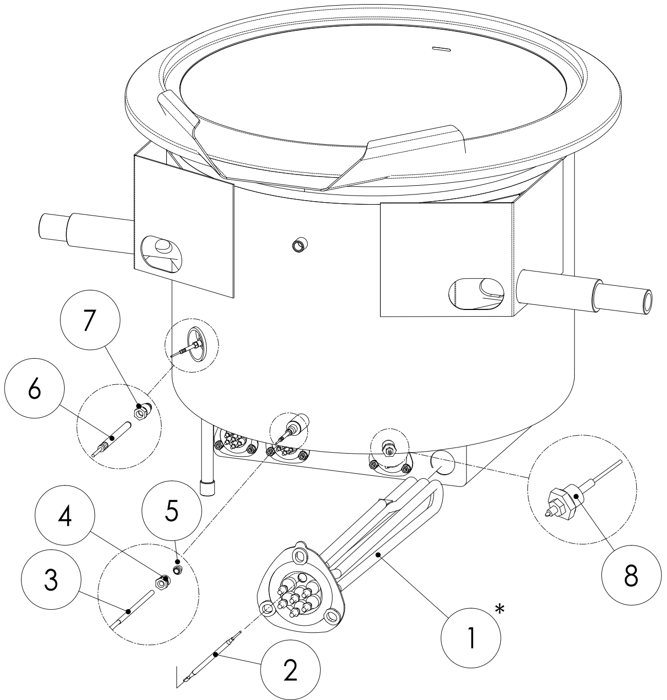
* TABLE HEATING ELEMENTS
