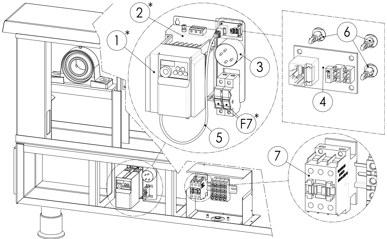
* TABLE INVERTER CODES, FILTER CODES AND FUSES (F7)
