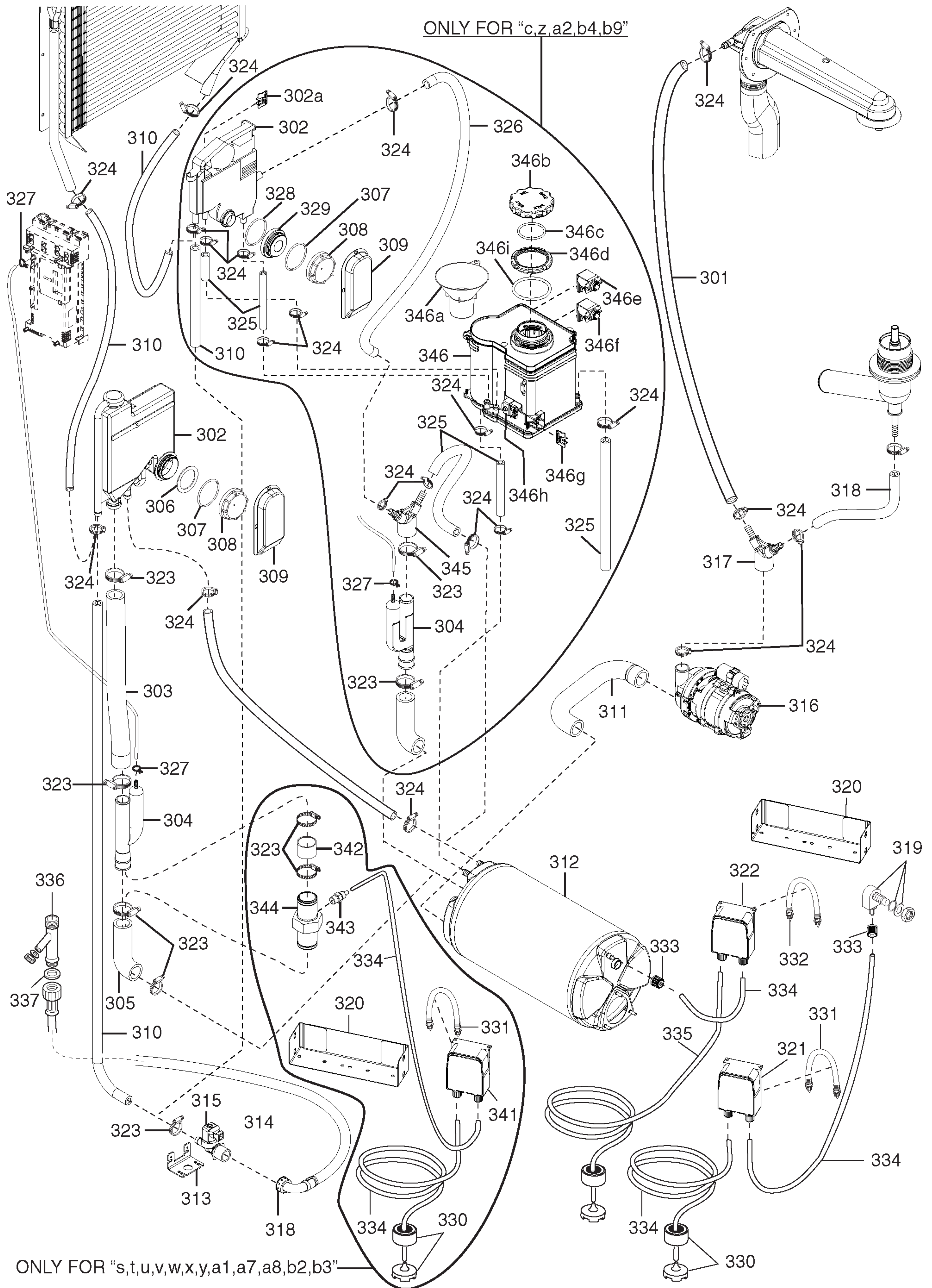
ill. 595668W00_p3 Circuito idraulico/ Hydraulic circuit
