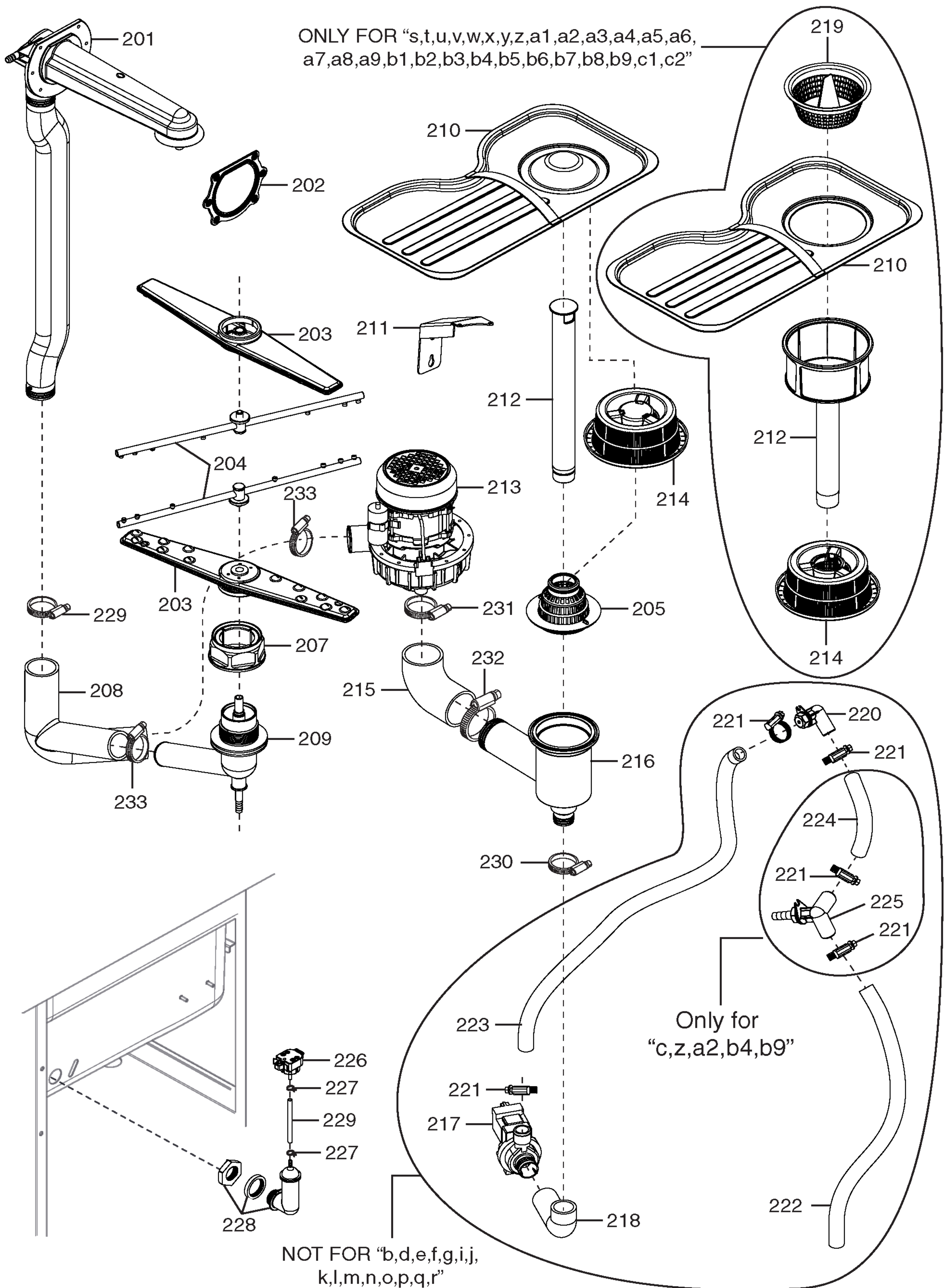
ill. 595668W00_p2 Componenti idraulici / Hydraulic components
